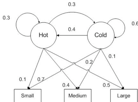
Figure 13: HMM Model
