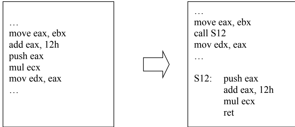
Figure 9: Subroutine Outlining
