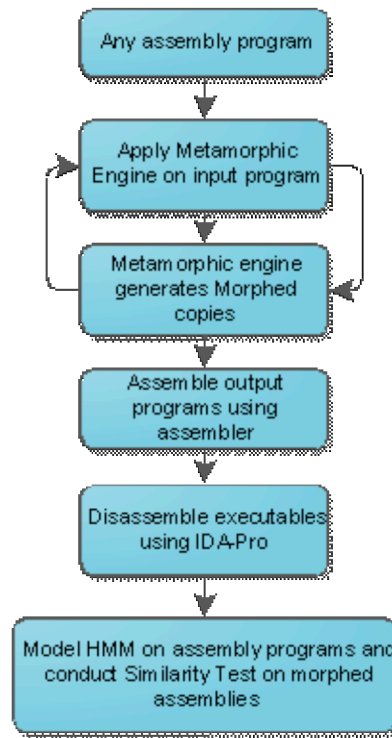
Figure 20: Overall Process
