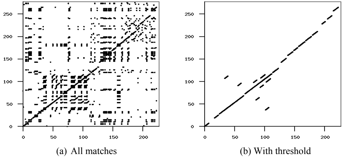
Figure 10: Similarity Graph
