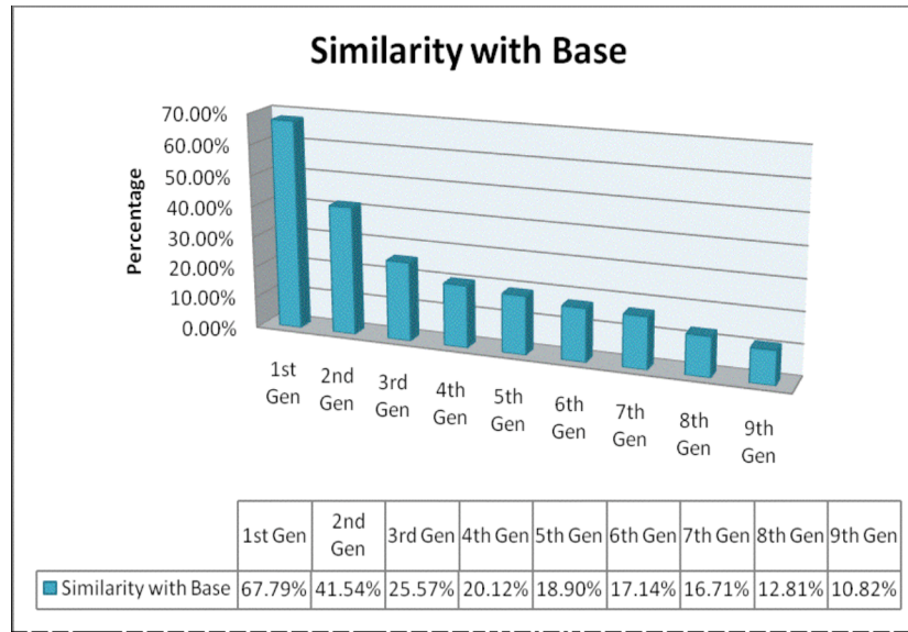
Figure 21: Similarity results of the base virus v/s 9 different generations
