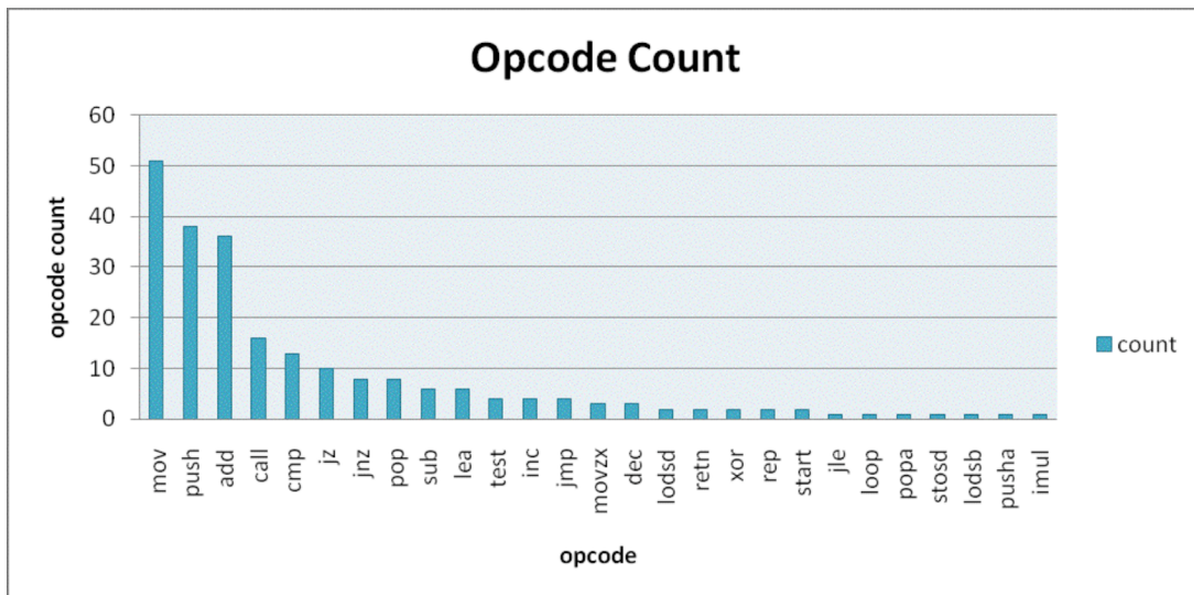
Figure 16: Base virus opcodes and their frequency
