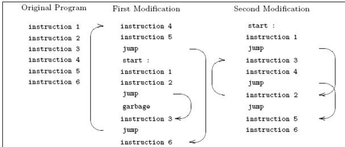
Figure 7: Example of control flow modification [15]
