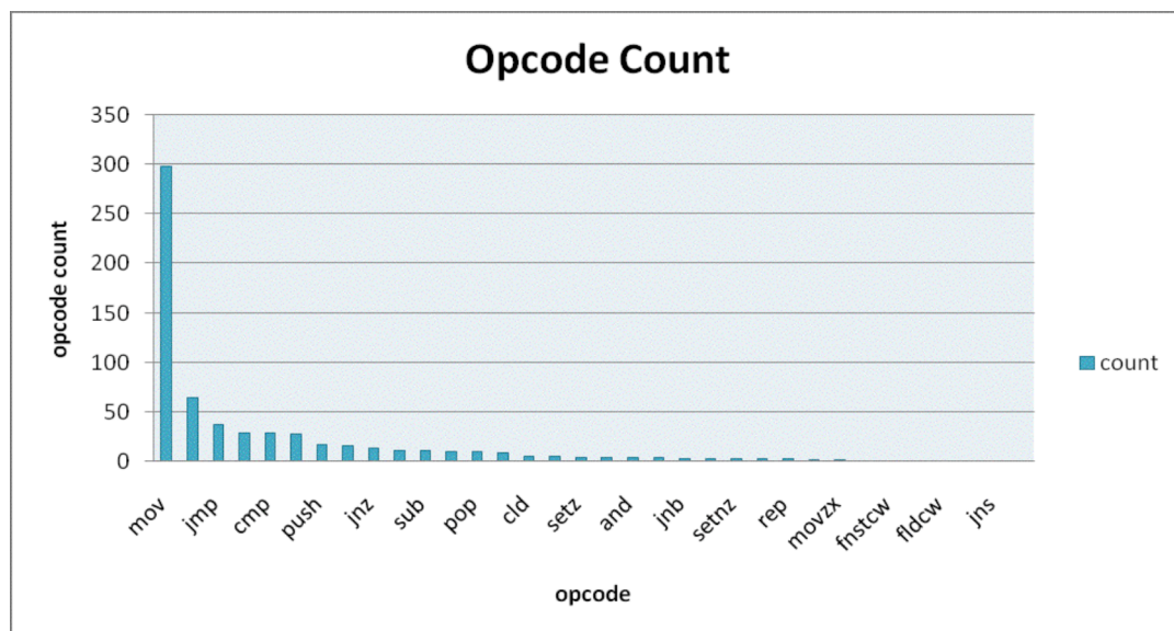
Figure 17: Opcodes of normal file and their frequency
