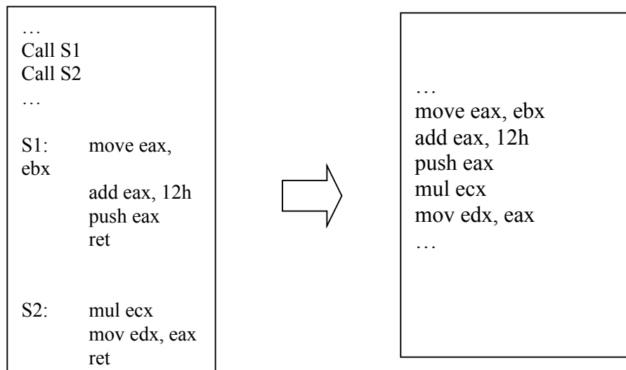
Figure 8: Subroutine Inlining
