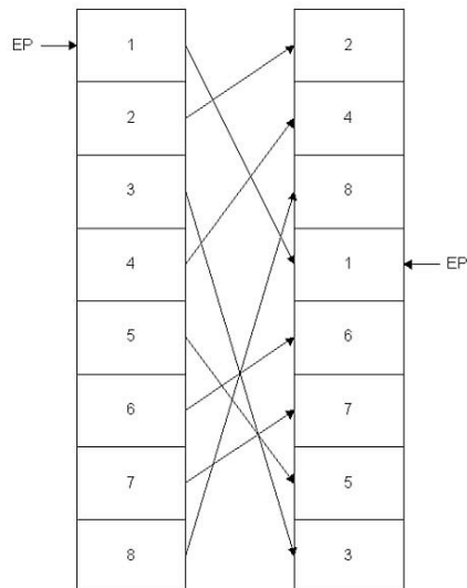
Figure 6: Subroutine permutation [4]
