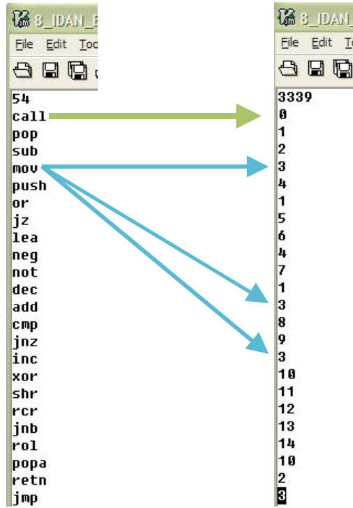
(a) Unique Symbols (b) Observation sequence
