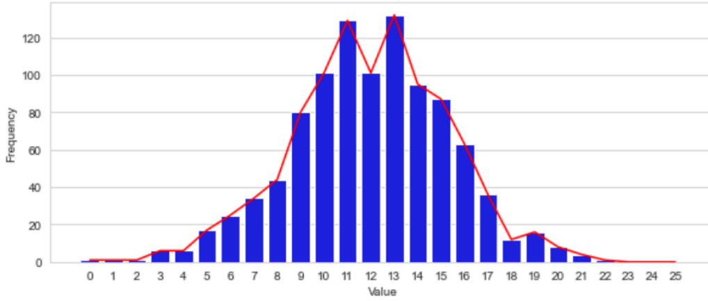
Normal Distribution, count = 1000000
