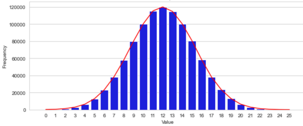
Normal Distribution, count = 1000000
