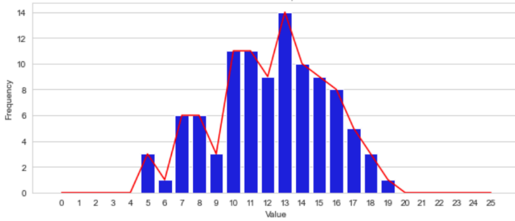
Normal Distribution, count = 100
