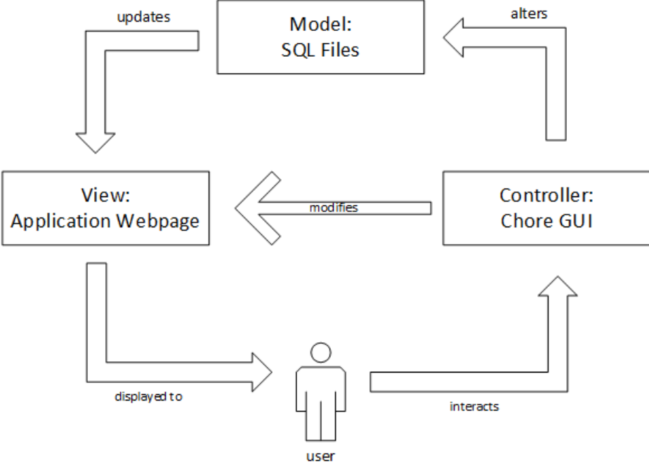
MVC Architecture
