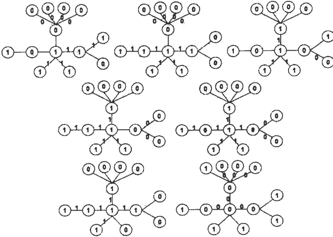
Figure 11: Balance index set of CT(1, 3, 2)(u_b(0, 0, 4))
