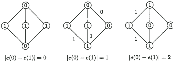
Figure 1: The friendly labelings of a graph G with \text{BI}(G) = \{0, 1, 2\} .
