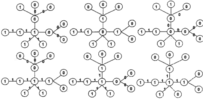
Figure 10: Balance index set of CT(1, 3, 2)(u_b(0, 0, 3))
