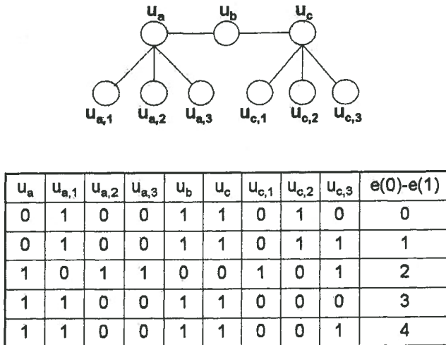
Figure 7: The balance index set of CT(3, 0, 3)
