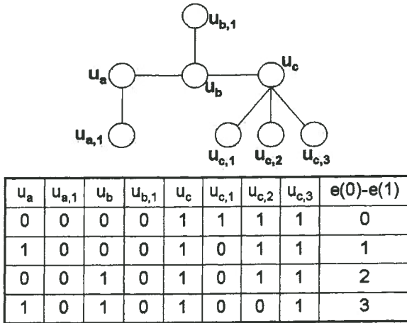
Figure 6: The balance index set of CT(1, 1, 3)
