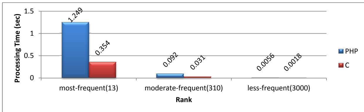
Chart 7 Encoding Test Results for 10,000 documents (PHP7, 32 bit, i7)
