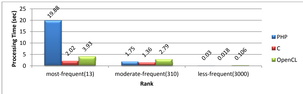
Chart 11 Decoding Test Results for 10,000 documents (PHP5, 32 bit, i7+Nvidia Graphics)
