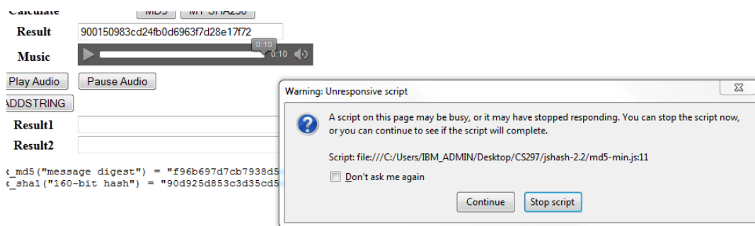
Figure 11: Browser stop
