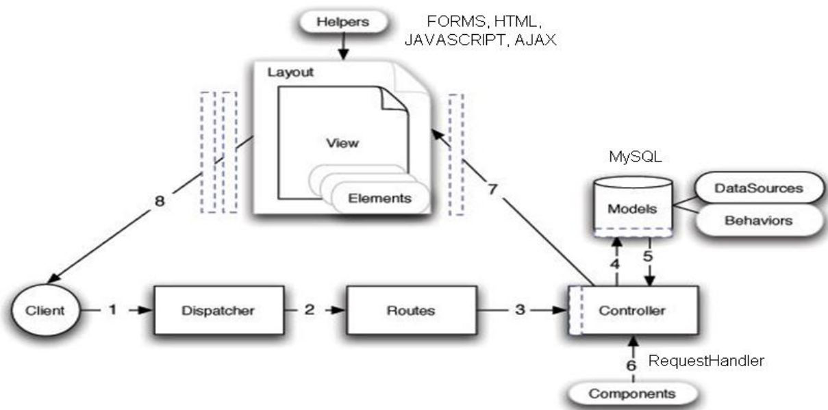
Figure 4. CakePHP Architecture
