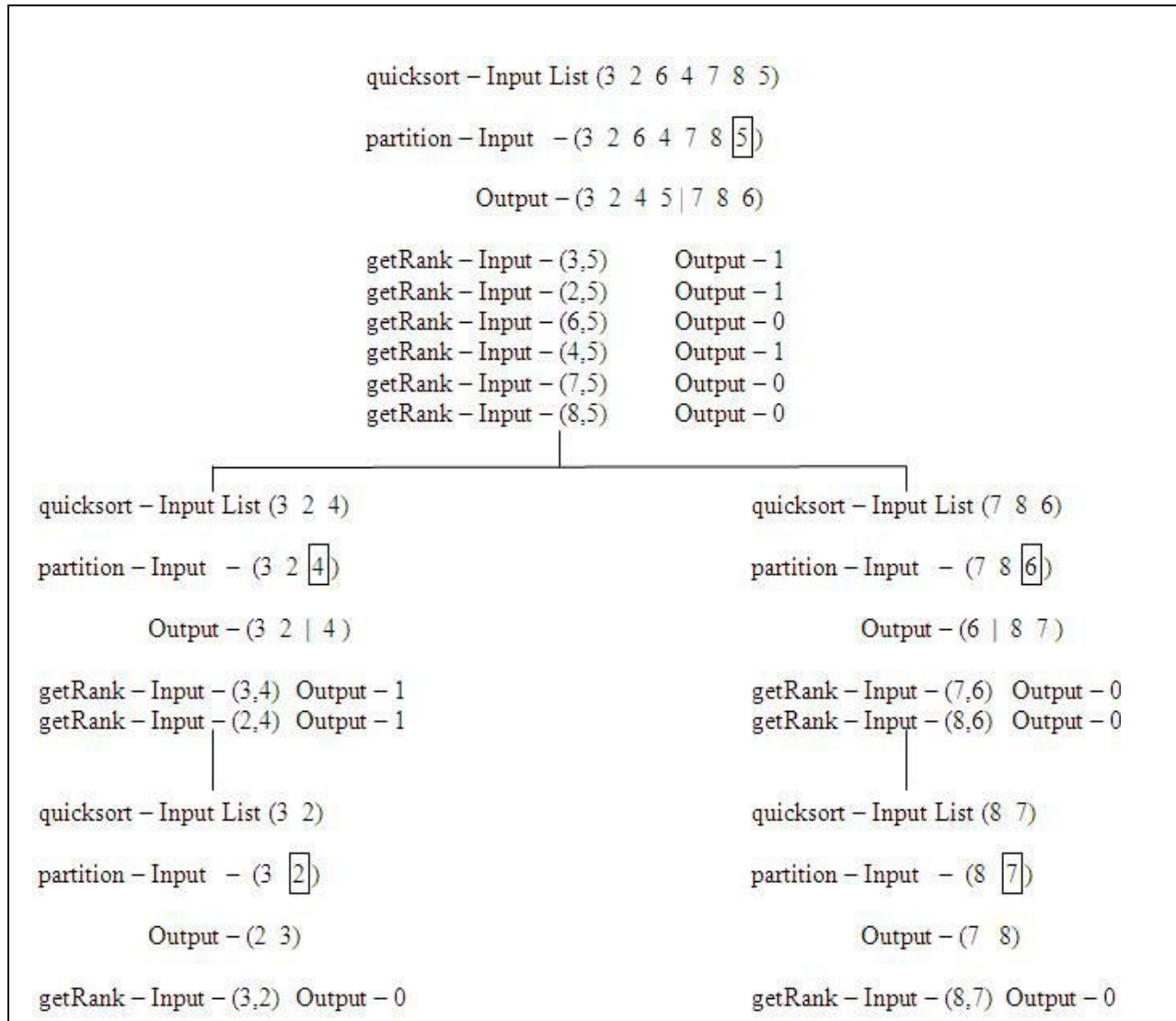
Fig 3. Partial Order QuickSort Example
