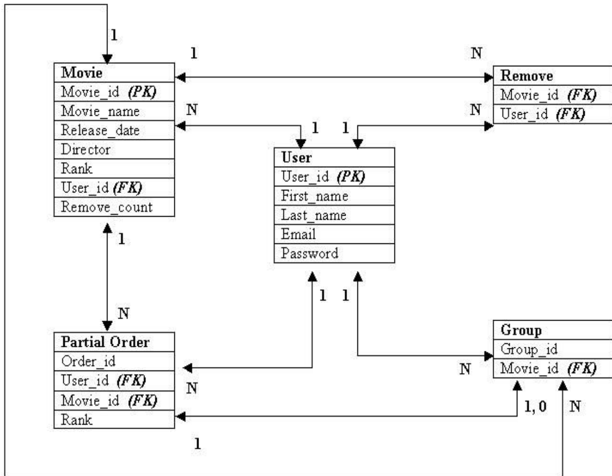
Fig 8. Entity-Relationship Diagram
