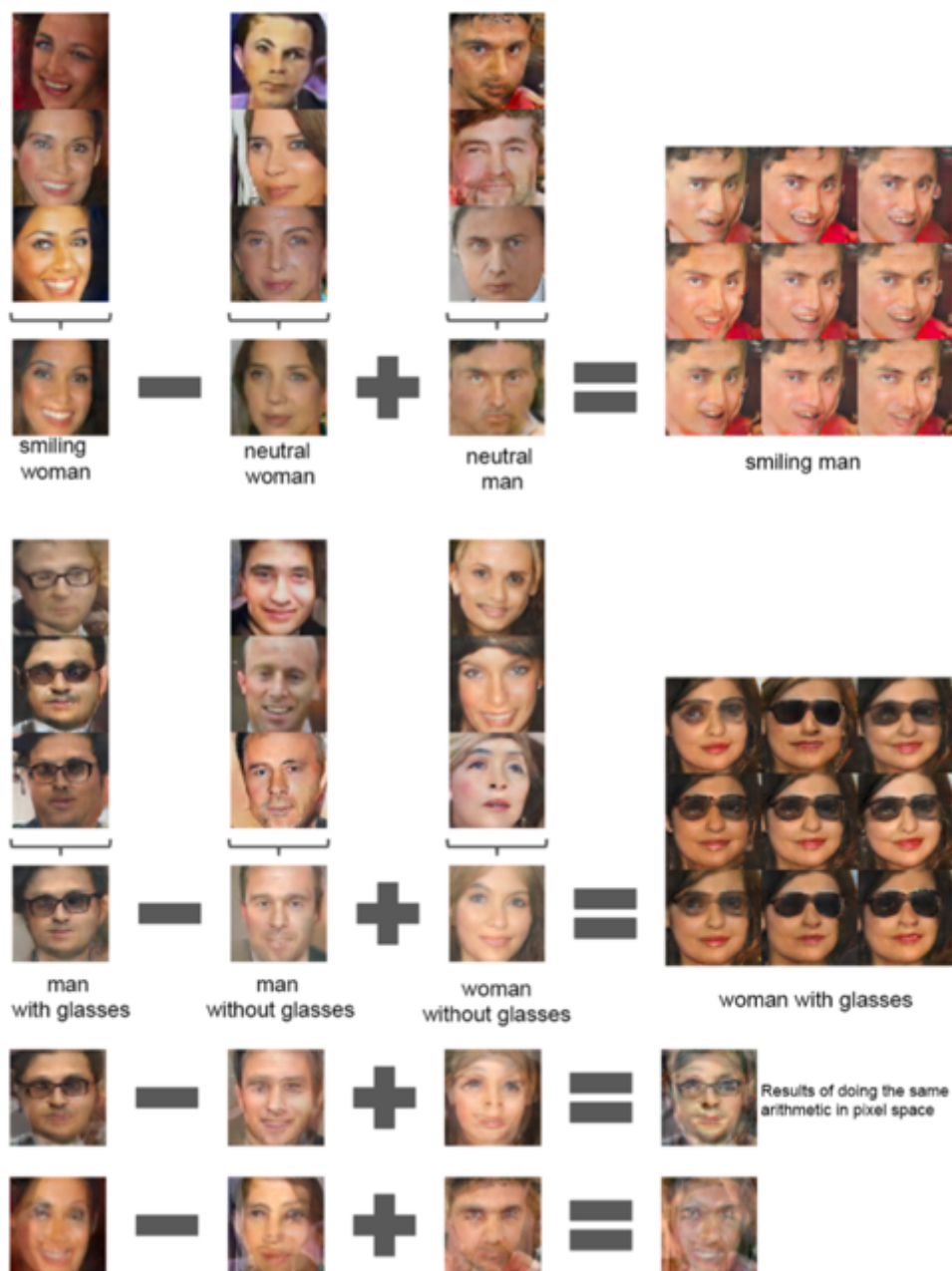
Figure 12: Vector arithmetic [19].
