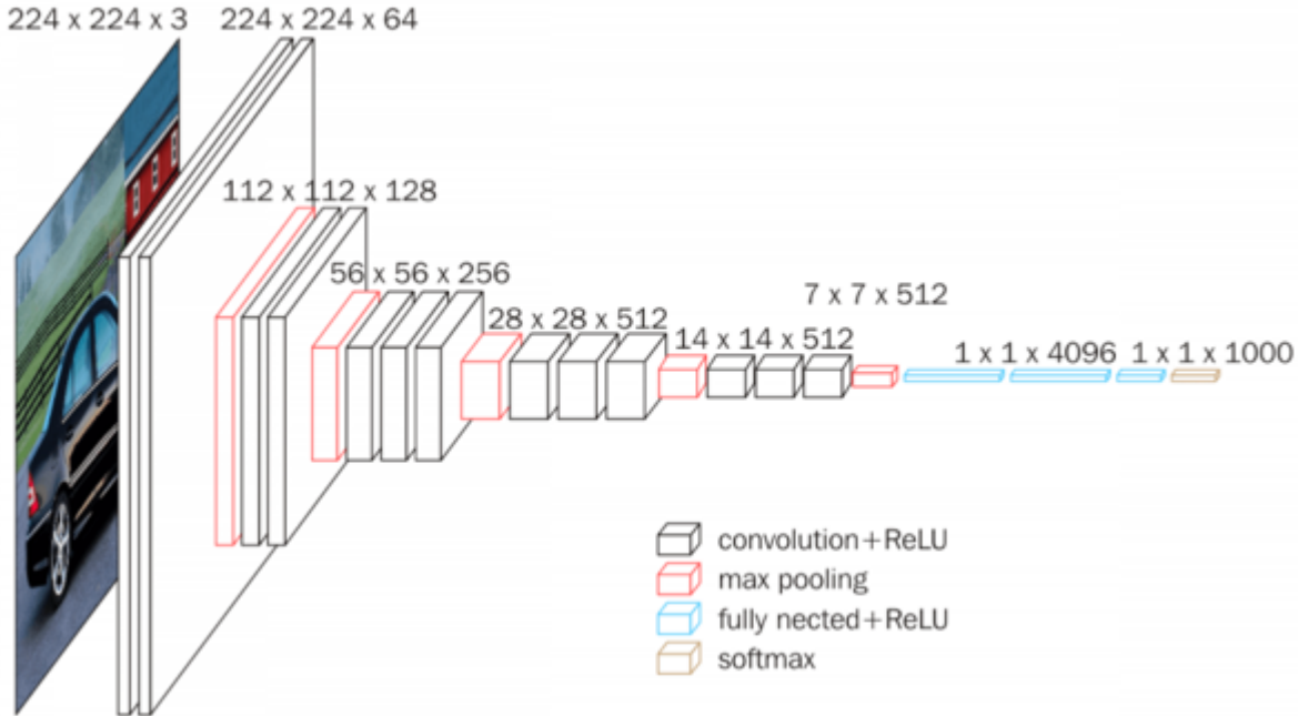
Figure 8: VGG-16 architecture.
